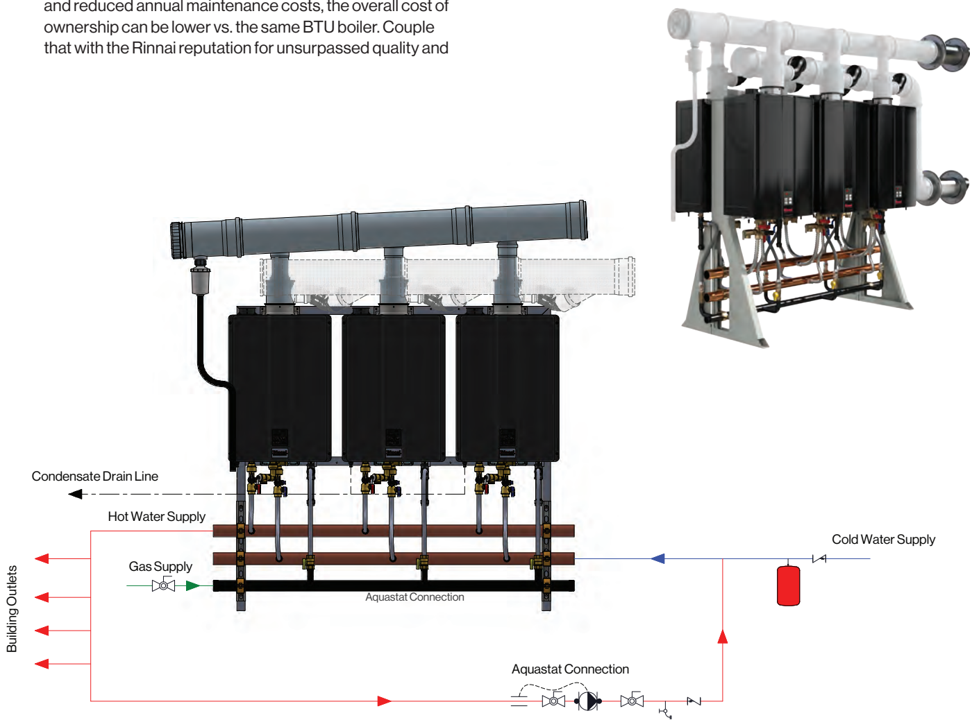
Simulated TRS with recirculation installation shown
